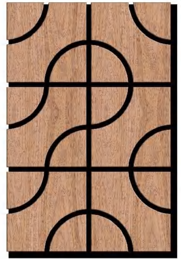
Item: HJ01TQ16 Material: HDF Black+PET Size: T 21mm x W 545mm x L 815mm
