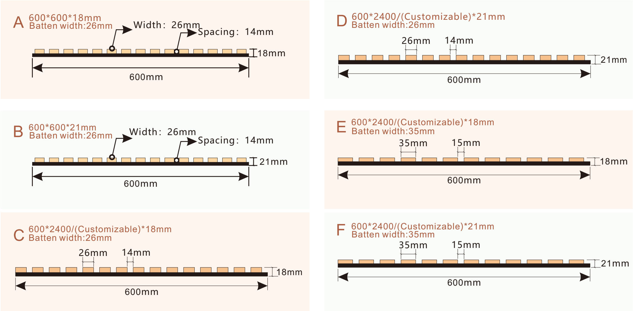
产品规格尺寸图解 DETAILED DRAWINGS OF PRODUCT DIMENSIONS
