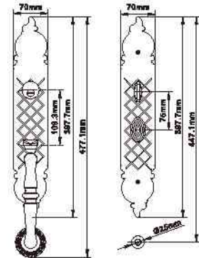
MODEL NO. : 8109 MATERIAL: Solid zinc alloy die-casting
