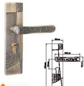
2918 DAB ET Supplying Finish: DAB, DAC, ORB, SG, YB. Lock Case Size: 45x50mm
