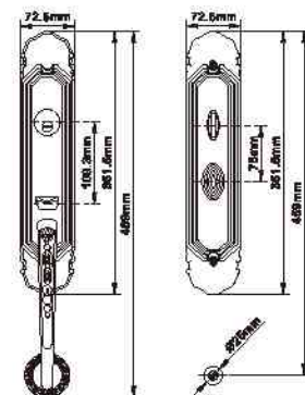
MODEL NO. : 8112 MATERIAL: Solid zinc alloy die-casting
