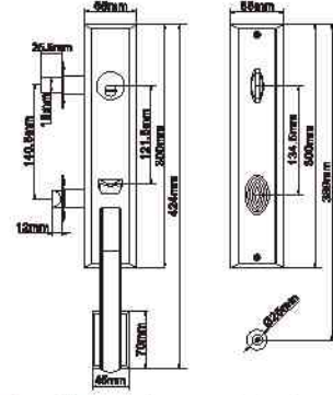
MODEL NO. : 8619 MATERIAL: Solid zinc alloy die-casting
