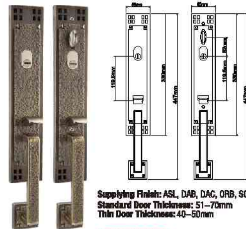
MODEL NO. : 8930-F MATERIAL: Solid zinc alloy die-casting
