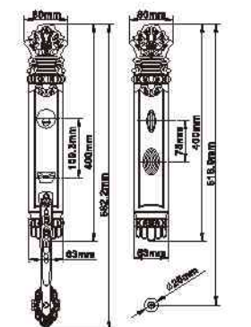
MODEL NO. : 8123 MATERIAL: Solid zinc alloy die-casting
