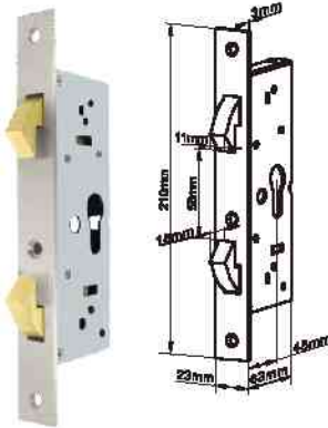
Series 82 ANSI/BHMA Grade 2 Lock Case
