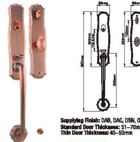
MODEL NO. : 8935-A MATERIAL: Solid zinc alloy die-casting
