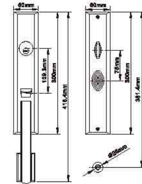
MODEL NO. : 8119 MATERIAL: Solid zinc alloy die-casting
