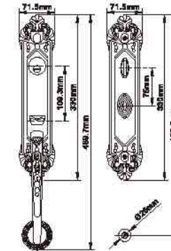
MODEL NO. : 8118 MATERIAL: Solid zinc alloy die-casting
