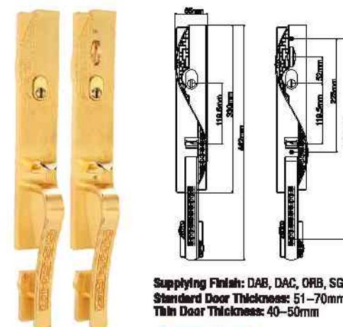
MODEL NO. : 8925-F MATERIAL: Solid zinc alloy die-casting
