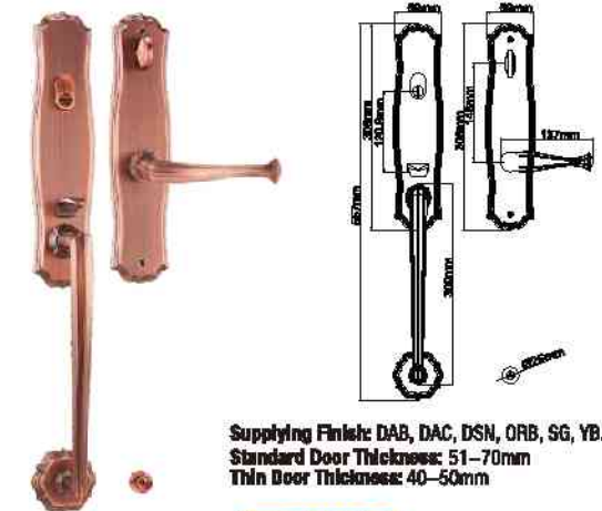
MODEL NO. : 8935-B MATERIAL: Solid zinc alloy die-casting
