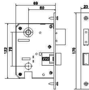
Backset Standard: 80mm(2 3/8") Customized: 70mm(2 3/4")
