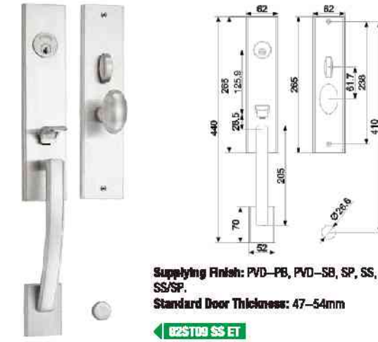
MODEL NO. : 82ST09 MATERIAL: Stamping stainless steel 304
