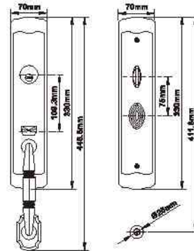
MODEL NO. : 8110 MATERIAL: Solid zinc alloy die-casting
