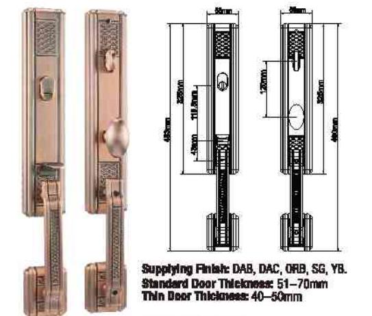
MODEL NO. : 8989-G MATERIAL: Solid zinc alloy die-casting
