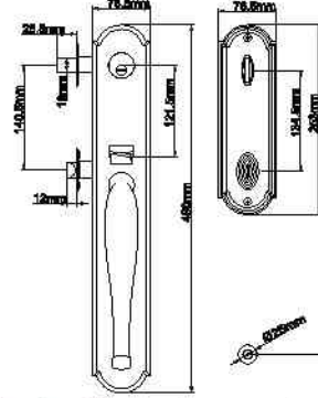
MODEL NO. : 8668 MATERIAL: Solid zinc alloy die-casting
