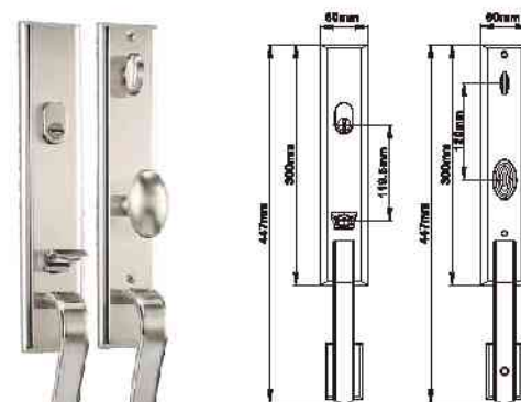
MODEL NO. : 8919-G MATERIAL: Solid zinc alloy die-casting
