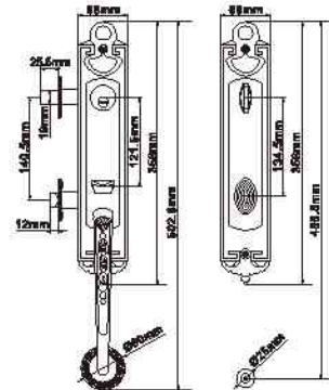
MODEL NO. : 8616 MATERIAL: Solid zinc alloy die-casting
