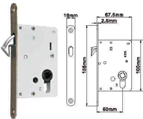
Series 550 Lock Case
