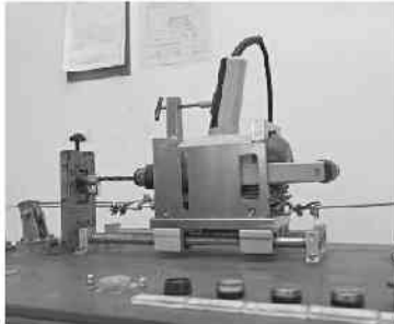
Anti-drill Test For Cylinder
