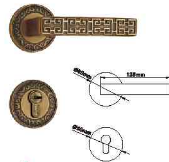
22B11 DAB ET Supplying Finish: AB, AC, DAB, DAC, QAC, ORB, PVD-PB, SG. Lock Case Size: 45x85mm
