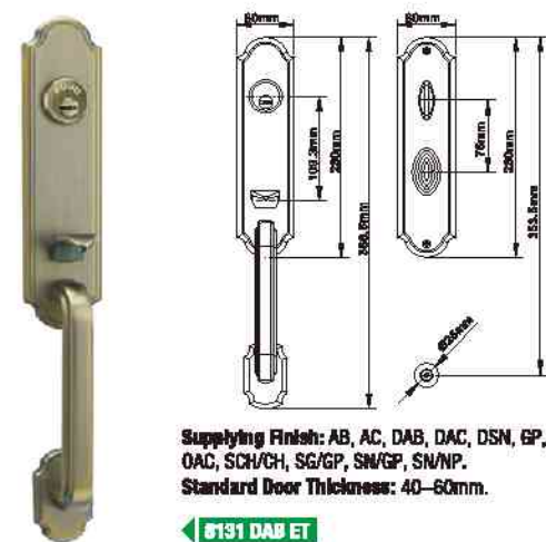
MODEL NO. : 8131 MATERIAL: Solid zinc alloy die-casting
