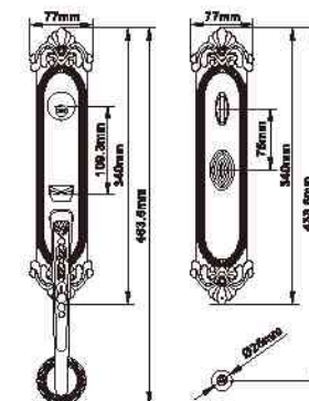
MODEL NO. : 8121 MATERIAL: Solid zinc alloy die-casting
