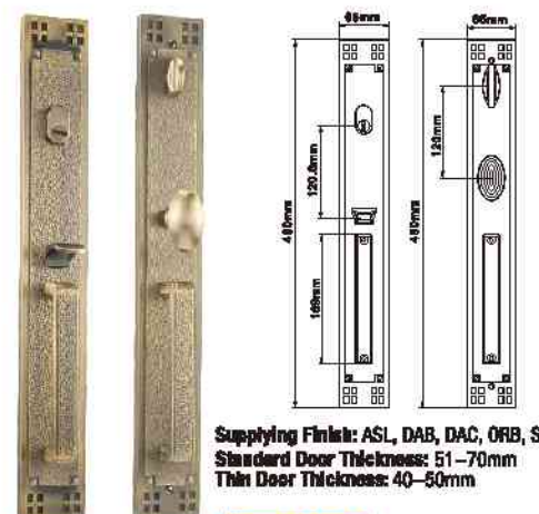
MODEL NO. : 8930-J MATERIAL: Solid zinc alloy die-casting
