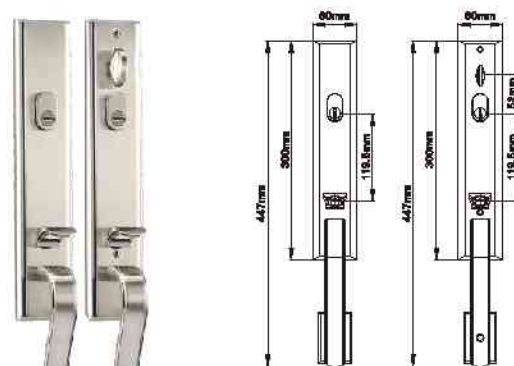
MODEL NO. : 8919-F MATERIAL: Solid zinc alloy die-casting
