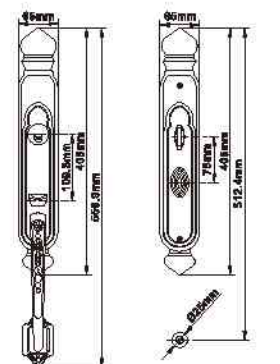
MODEL NO. : 8115 MATERIAL: Solid zinc alloy die-casting
