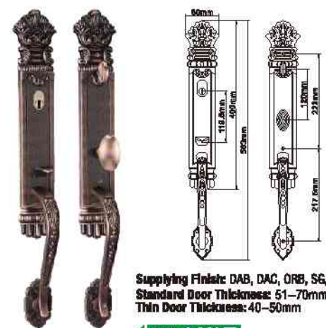
MODEL NO. : 8923-G MATERIAL: Solid zinc alloy die-casting
