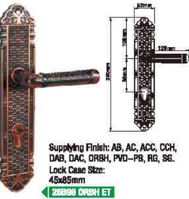
MODEL NO. : 26B98 MATERIAL: Solid forged brass
