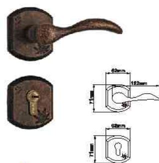
22B33 ACC ET Supplying Finish: AB, AC, ACC, CCH, DAB, DAC, DSN, ORBH, PVD-PB, RG, SG, SN. Lock Case Size: 80x85mm
