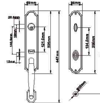
MODEL NO. : 8623 MATERIAL: Solid zinc alloy die-casting
