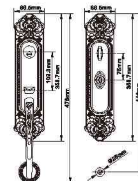
MODEL NO. : 8120 MATERIAL: Solid zinc alloy die-casting
