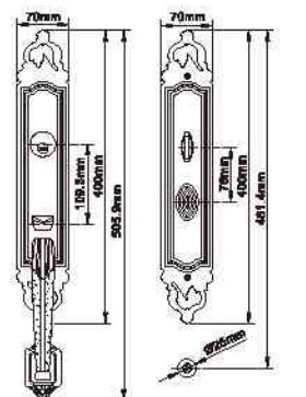
MODEL NO. : 8113 MATERIAL: Solid zinc alloy die-casting
