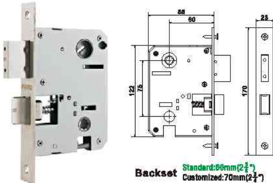
81 Series Lock Case
