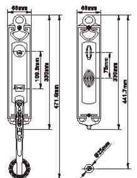
MODEL NO. : 8116 MATERIAL: Solid zinc alloy die-casting
