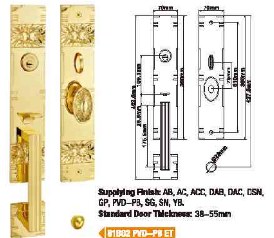
MODEL NO. : 81B02 MATERIAL: Solid forged brass
