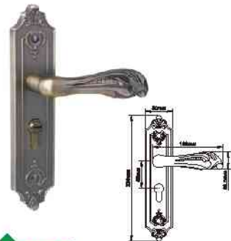
2915 DAB ET Supplying Finish: DAB, DAC, ORB, SG, YB. Lock Case Size: 45x50mm
