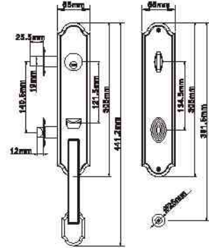
MODEL NO. : 8621 MATERIAL: Solid zinc alloy die-casting
