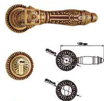
22B22 RG ET Supplying Finish: AB, AC, CCH, DAB, DAC, ORBH, PVD-PB, RG, SG. Lock Case Size: 45x85mm
