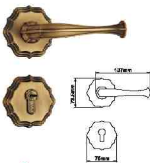
22B10 DAB ET Supplying Finish: AB, AC, DAB, DAC, QAC, ORB, PVD-PB, SG. Lock Case Size: 60x85mm
