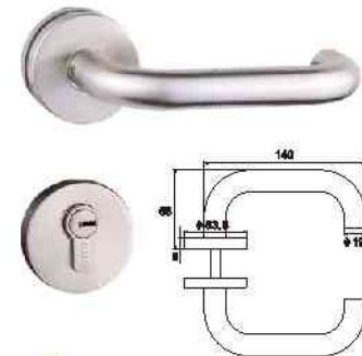
2250 SS ET Supplying Finish: SS Lock Case Size: 45x85mm
