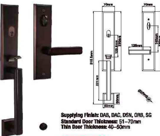
MODEL NO. : 8988-B MATERIAL: Solid zinc alloy die-casting
