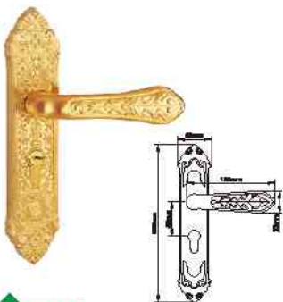
2912 SG ET Supplying Finish: DAB, DAC, ORB, SG, YB. Lock Case Size: 45x50mm
