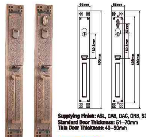
MODEL NO. : 8930-H MATERIAL: Solid zinc alloy die-casting
