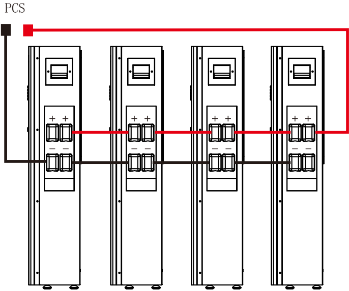
Multi-Units Connection
