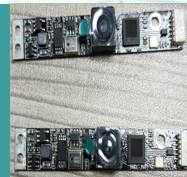
教育大屏摄像头 Educational large screen camera
