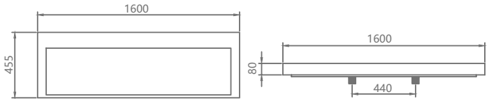
KKR-1265-2 Size: 1600x455x80mm
