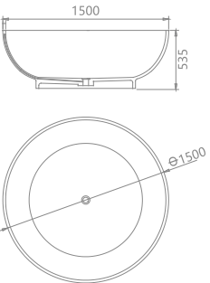
KKR-B002-C Size:1500x1500x535mm
