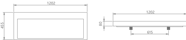
KKR-1264 Size: 1202x455x80mm
