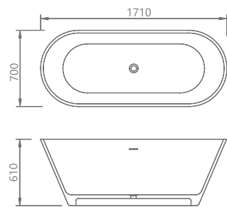
KKR-B050 Size: 1710x700x610mm
