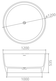
KKR-B002-B Size: Dia1200x535mm
