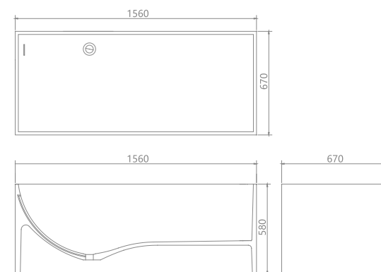
KKR-B029-A Size:1560x670x580mm
