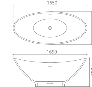
KKR-B051-B Size: 1650x730x640mm
