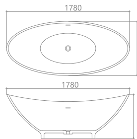
KKR-B051-A Size: 1780x785x590mm
