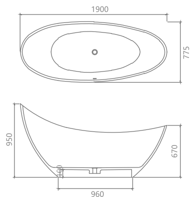
KKR-B072 Size: 1900x775x950mm
