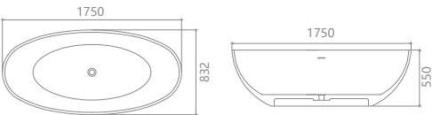
KKR-B008-B Size: 1750x832x550mm
