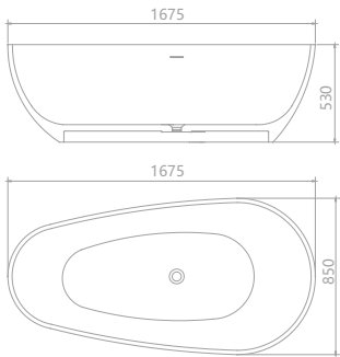
KKR-B001 Size: 1675x850x530mm
