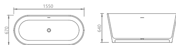
KKR-B047 Size: 1550x670x640mm
