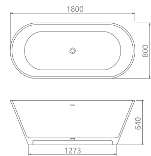
KKR-B050-A Size: 1800x800x640mm
