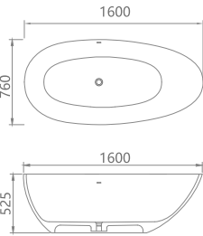
KKR-B068-A Size: 1600x760x525mm
