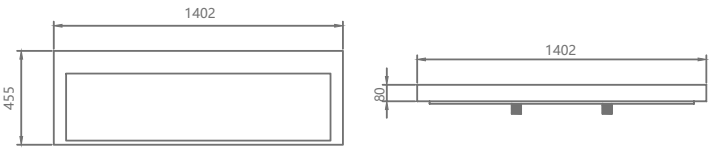
KKR-1265 Size: 1402x455x80mm
