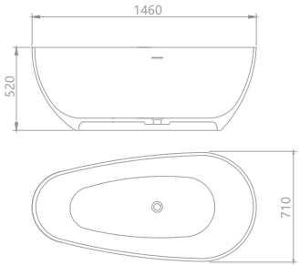
KKR-B001-A Size:1460x710x520mm
