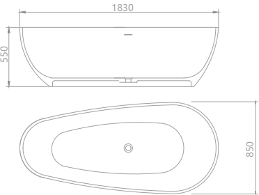
KKR-B001-B Size:1830x850x550mm
