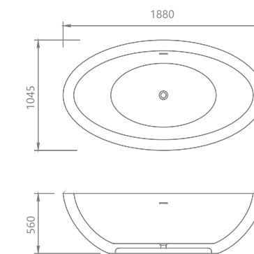
KKR-B048 Size: 1880x1045x560mm
