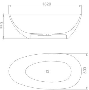
KKR-B001-C Size:1620x800x550mm
