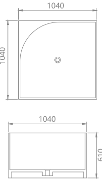
KKR-B067 Size: 1040x1040x610mm
