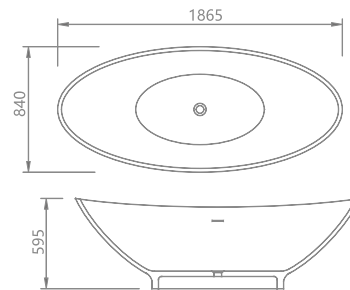
KKR-B051 Size: 1865x840x595mm
