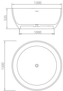
KKR-B002-A Size: Dia1300x535mm
