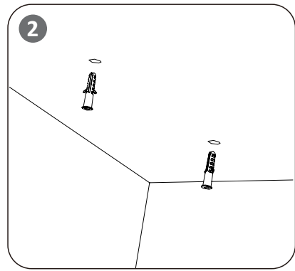
Drive the expansion screw into the drilled hole
