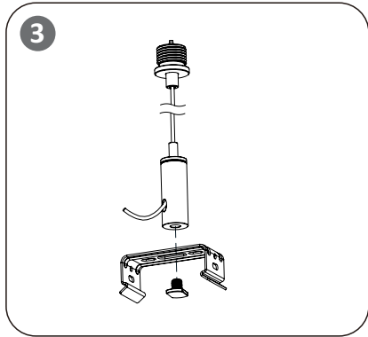
Press the buckle tightly on the back of the lamp
