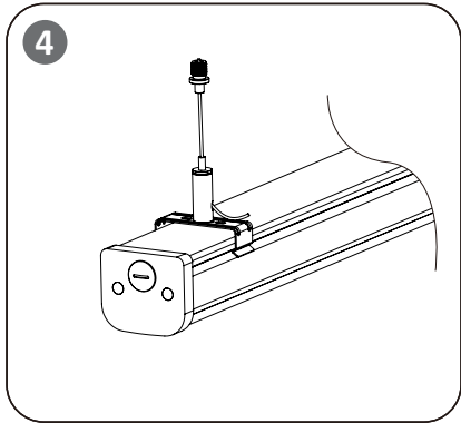
Fix the expansion screw and the female buckle on the ceiling by screws
