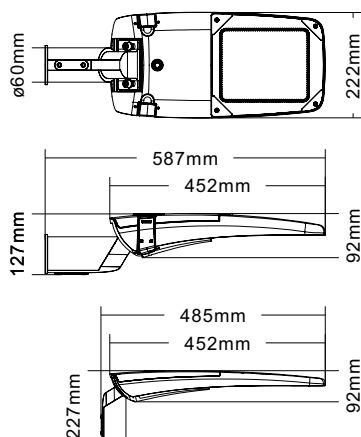
ST42-S (20W / 30W / 40W / 50W / 60W / 80W)
