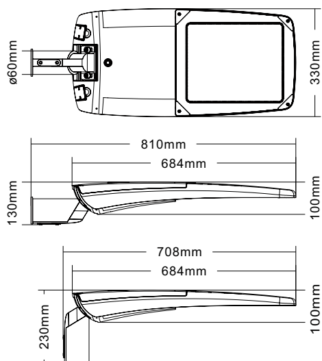
ST42-L (180W / 200W / 210W / 240W / 250W)
