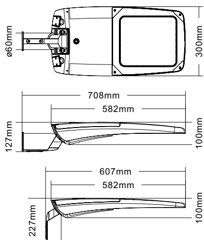
ST42-M (100W / 110W / 120W / 150W / 160W)
