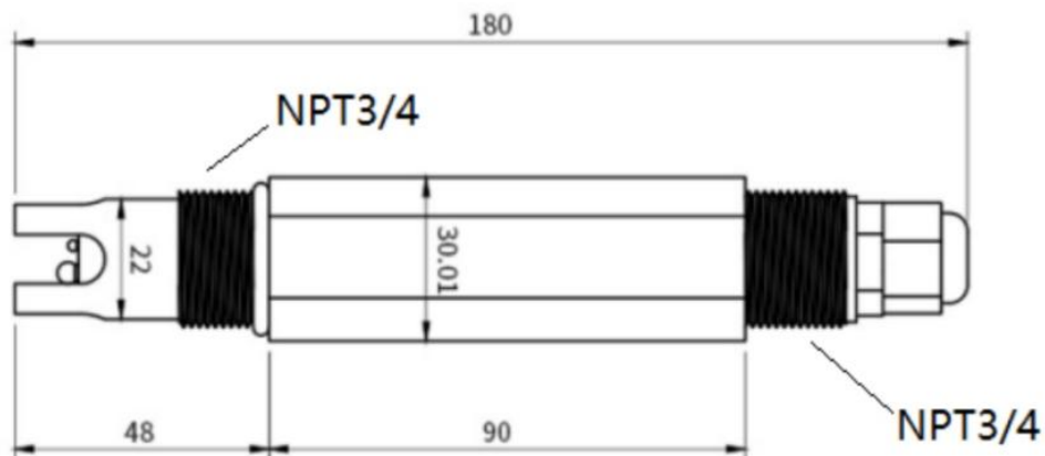
Figure 5.1 Dimension Specification
