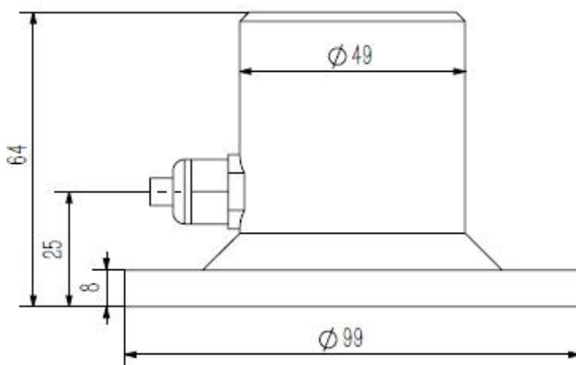
Figure 6.3 Side view with protective dome
