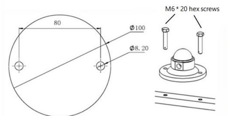
Figure 8.1.1 Tilted Installation Compatible with RK95-56 Bracket(Unit:mm)
