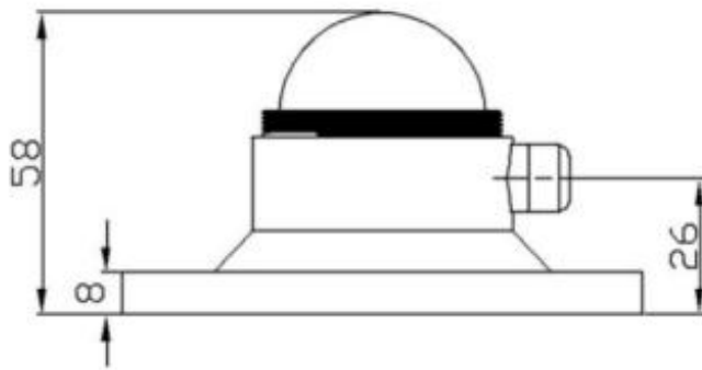
Figure 6.1 Side view
