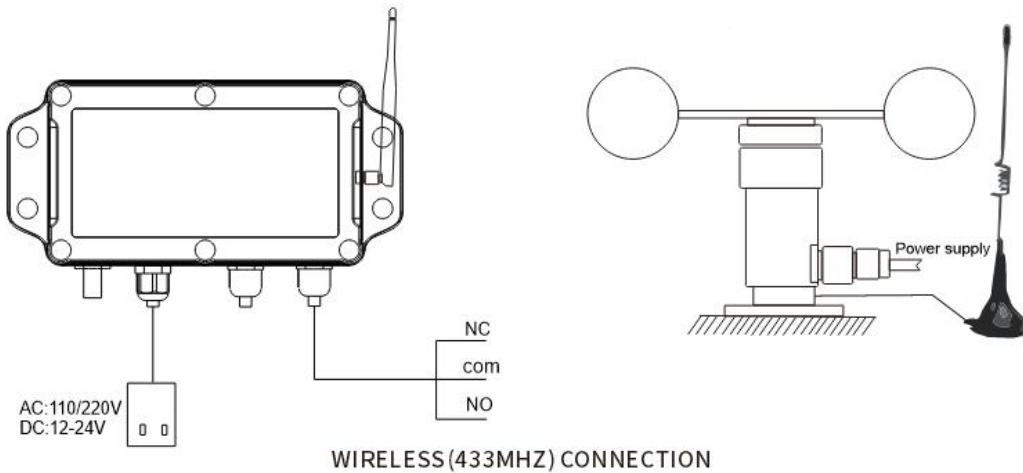
Figure 8.1.2 Wireless (433MHz) Connection for Wind Speed Sensor
