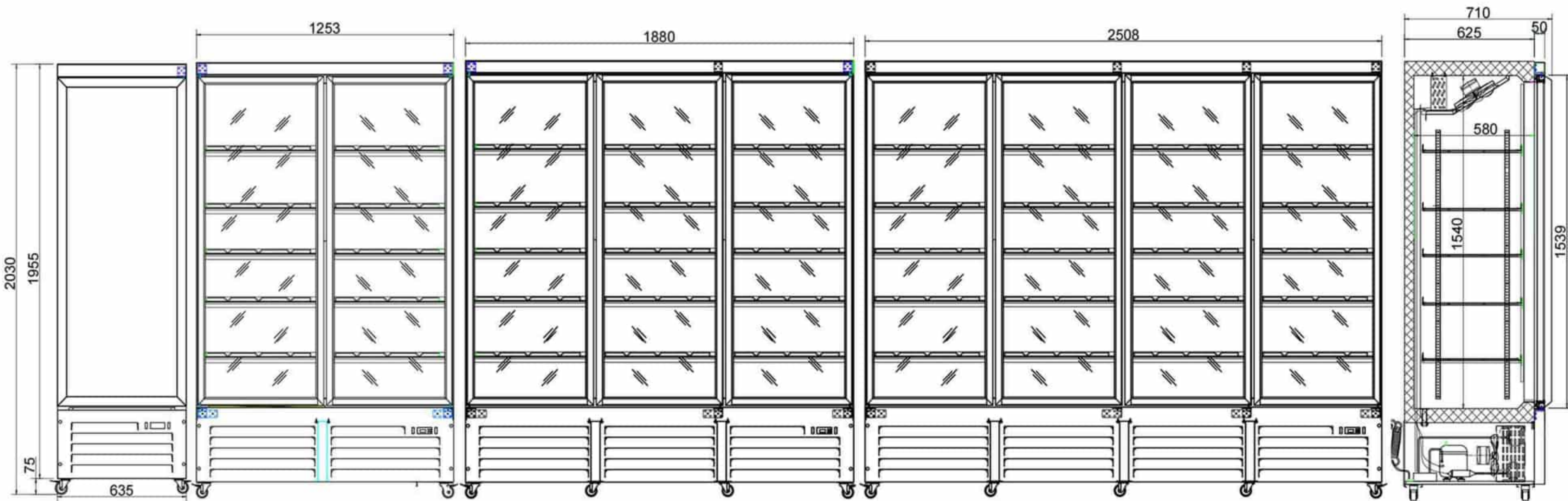
PRODUCT DRAWING
