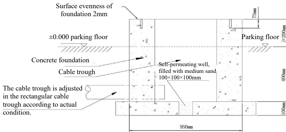
Foundation section
