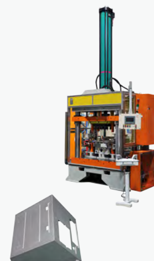
75T 电器外壳铆接机 75T Clinch Machine For Electric Cover
