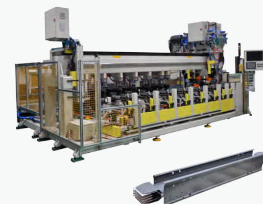
母线自动装配铆接机 Automatic Assembly Clinch Machine For The Aluminum Bus Bar
