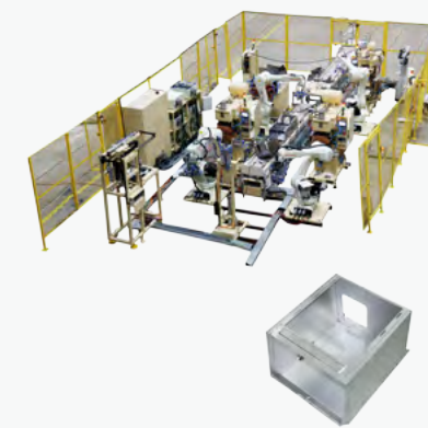
抽油烟机箱体铆接生产线 Automatic Welder For Range Hood
