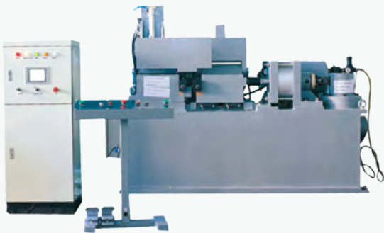
150KVA 杠杆加压式闪光对焊机 150KVA flash Butt Welder With Hydraulic Toggle Clamping Head ZUN-150-012-0001
