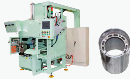
主壳体三点弧焊机 Main Housing Three-Point Arc Welding Machine
