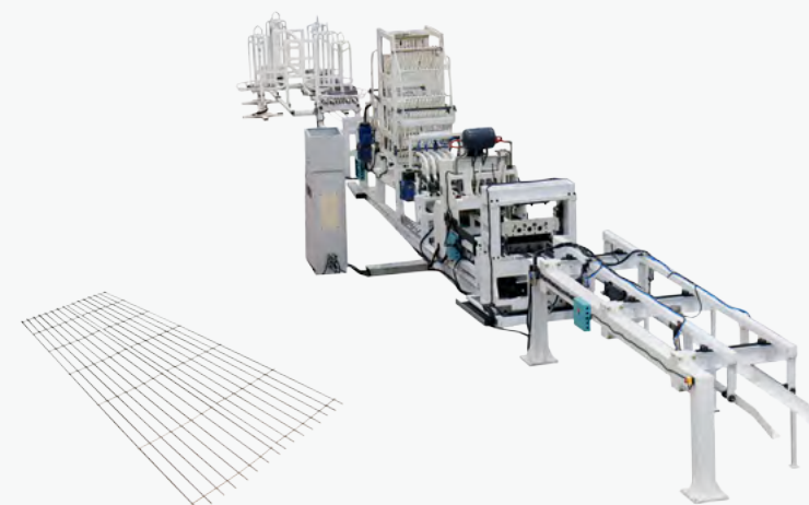
200KVA 加气墙体骨架铁线网自动焊机 200KVA Automatic Multi Spot Welder With Wire Feeder For Preformed Wall Frame
