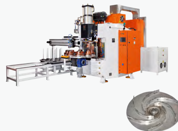
60000J 水泵叶片八工位中压储能焊机 60000J CD Welder For Water Pump Vane With 8 Station
