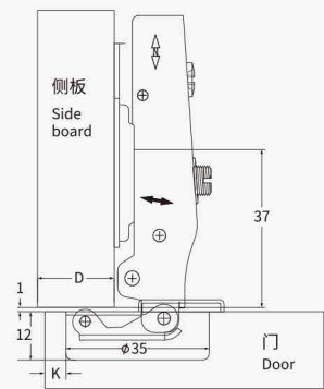
全盖 Full overlay
