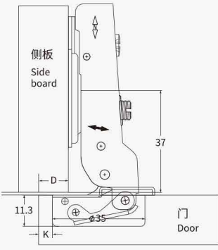
半盖 Half overlay
