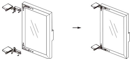
1. 左右方向调节 Left and right adjustment
