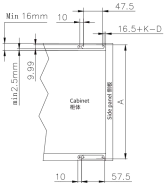
柜体开孔尺寸图 Cabinet drilling dimension picture
