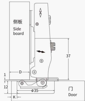
全盖 Full overlay
