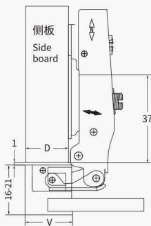
全盖 Full overlay
