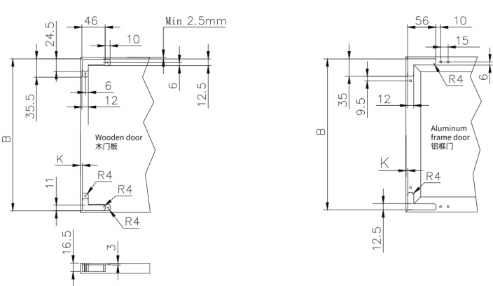
木门和铝门框开孔尺寸图 Wood door and aluminum door drilling dimension picture
