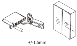
1. 左右方向调节 Left and right adjustment
