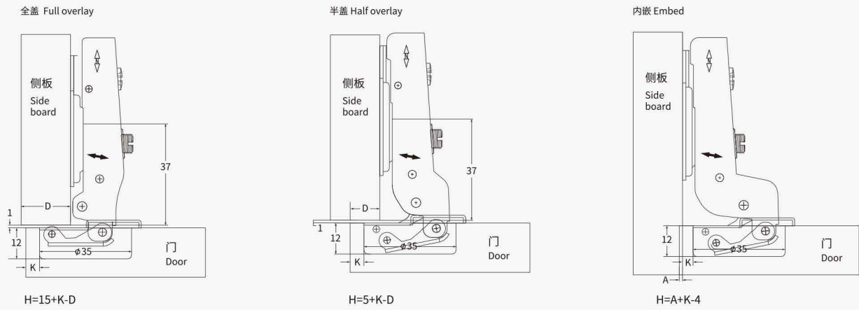
D: 盖位计算值表/overlay calculation form
