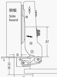
半盖 Half overlay
