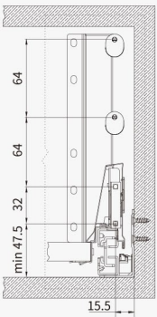
前接码面板安装尺寸 Front connector panel installation dimensions
