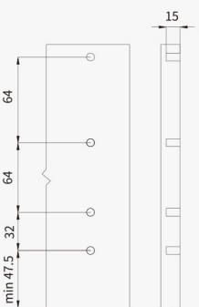
面板钻孔尺寸 Front panel drilling dimensions
