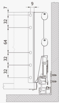
背板安装尺寸 Back panel installation dimensions
