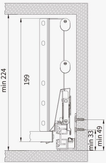
柜体所需空间 Cabinet space requirements
