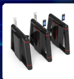
BLS-NF318 (Flap barrier gate) Size: 1400x280x980mm
