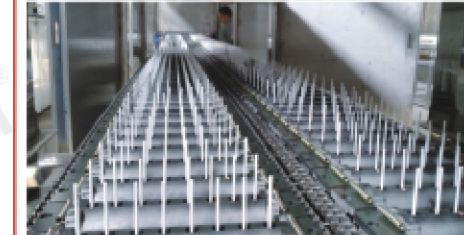
Automatic Stick Direct insertion System(BALL):SDS 自动直插式插棒系统(球形棒棒糖):SDS
