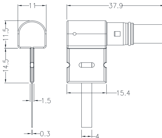
Edge side connector:EC1AF
