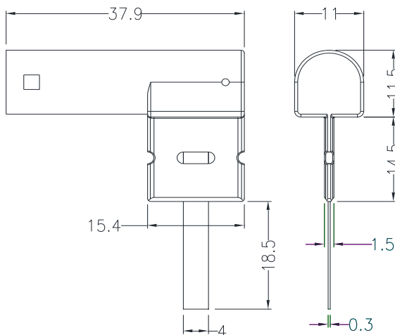
Edge side connector:EC1AM
