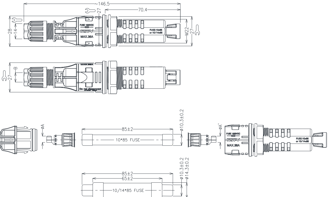
4PFC Panel fuse connector cable end
