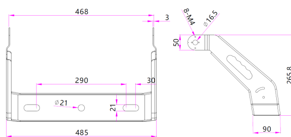
Bracket: KML-QC06-500/ KML-QC06-800
