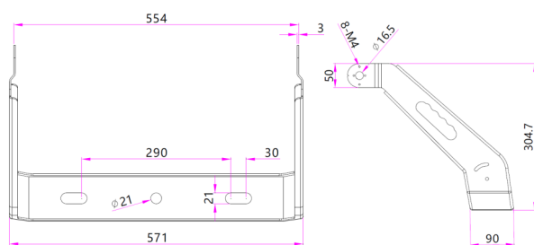
Bracket: KML-QC06-1000/ KML-QC06-1200
