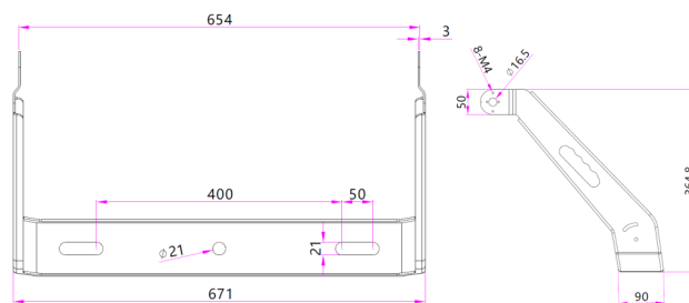
Bracket: KML-QC06-1500/ KML-QC06-1800
