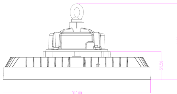
HB30-200 | HB30-240
