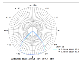
Type II-M PC lens
