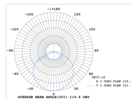
Type III-M PC lens
