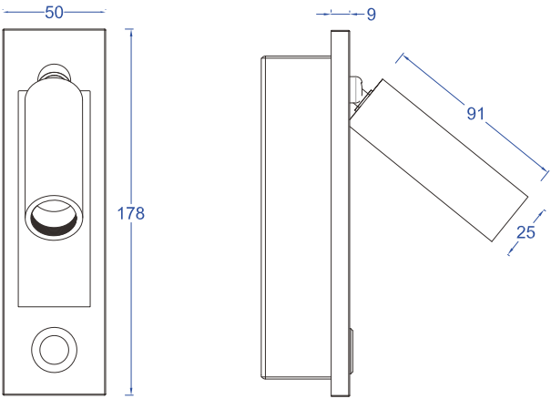
Cutout size:L160xW40xH60mm Unit:mm
