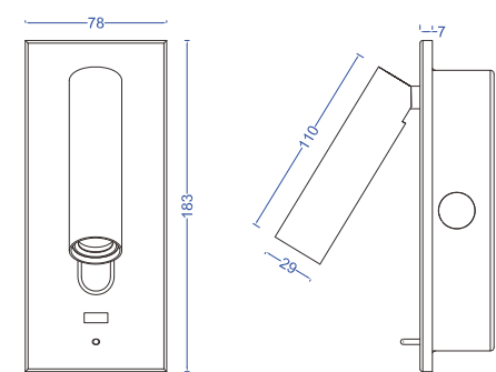
Cutout size : L155 x W55 x H40mm Unit:mm
