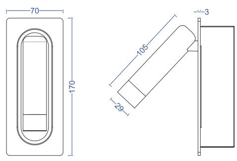
Cutout size : L150 x W55 x H45mm Unit:mm
