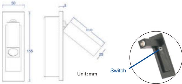
Cutout size : L130 x W40 x H50mm
