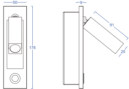
Cutout size: L160 x W40 x H60mm Unit:mm
