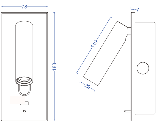
Cutout size : L155 x W55 x H40mm Unit:mm
