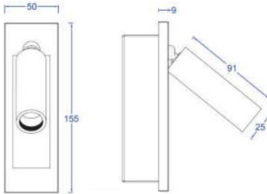
Cutout size : L130 x W40 x H50mm Unit:mm
