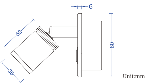
Cutout size : D50 x H50mm
