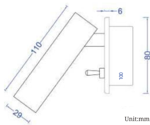
Cutout size : D70 x H50mm
