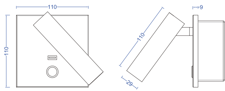
Cutout size : L95xW65 xH50mm Unit:mm
