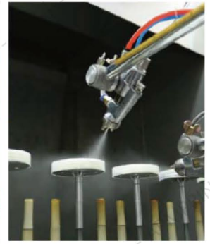
Automatic spraying (TOP coating)
