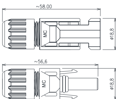
MC4 cable connector
