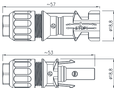
Newsun 1000VDC cable connector:
