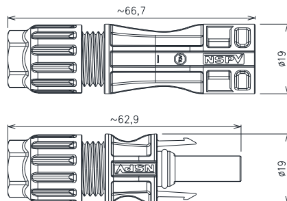
Newsun 1500VDC cable connector:
