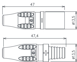
Newsun 1000VDC PV3.0 cable connector:
