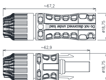
MC4_EVO cable connector
