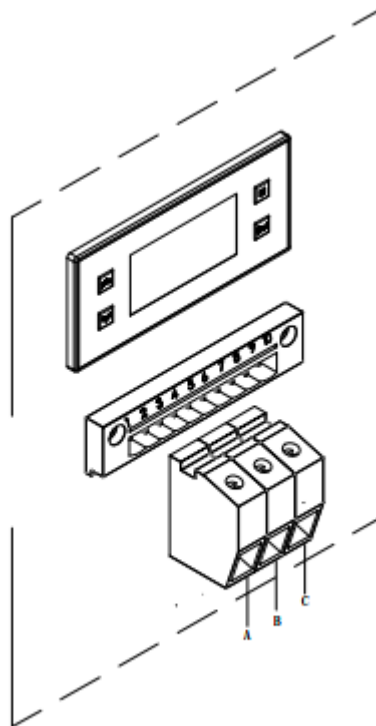
Figure 3-1 Schematic of power terminal
