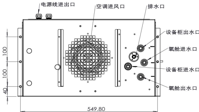
Figure 3-1 Schematic of power terminal
