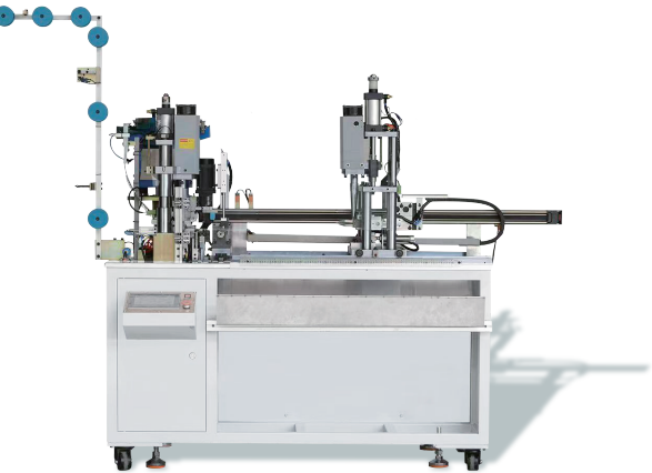
ZY-709N-D 全自动尼龙超音波五合一机 ZY-709N-D Full auto ultrasonic slider mounting double welding stops and cutting machine
