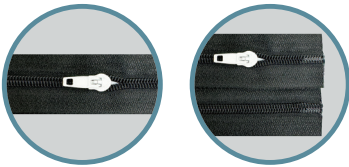
ZY-709N-D 全自动尼龙超音波五合一机 ZY-709N-D Full auto ultrasonic slider mounting double welding stops and cutting machine
