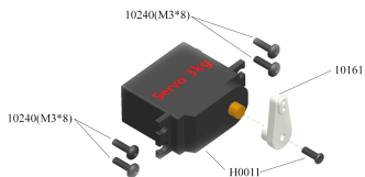
Steering Servo
