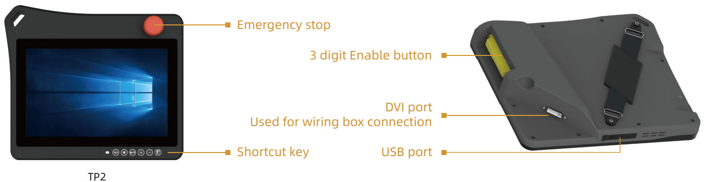
TP2
