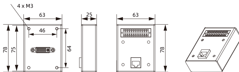
TP2-R2-JB wiring box size
