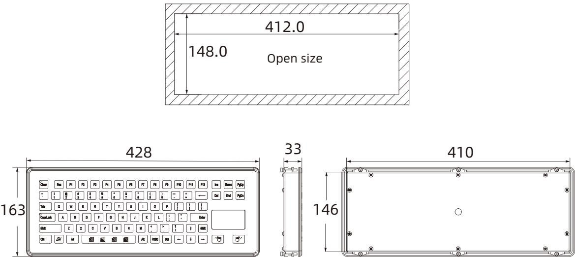
Panel Cutout Dimensions: 412mm x 148mm (16.22 x 5.83in)
