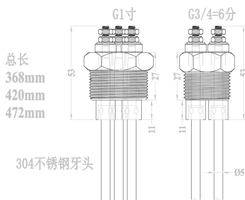
Electrode Probe Length
