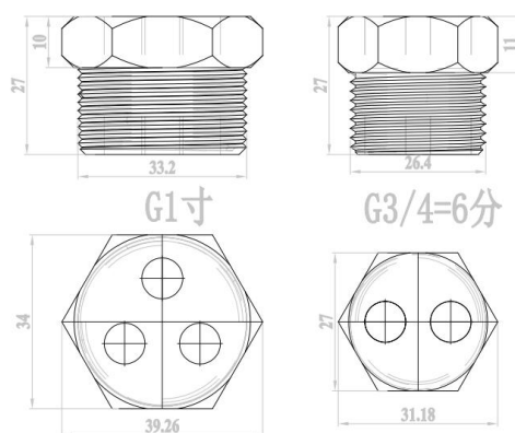
Fastening thread size
