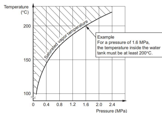
Operating temperature and pressure range
