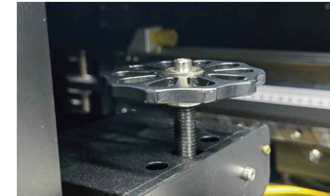
Rubber roller pressure knob, can flexibly adjust the pressure on both sides
