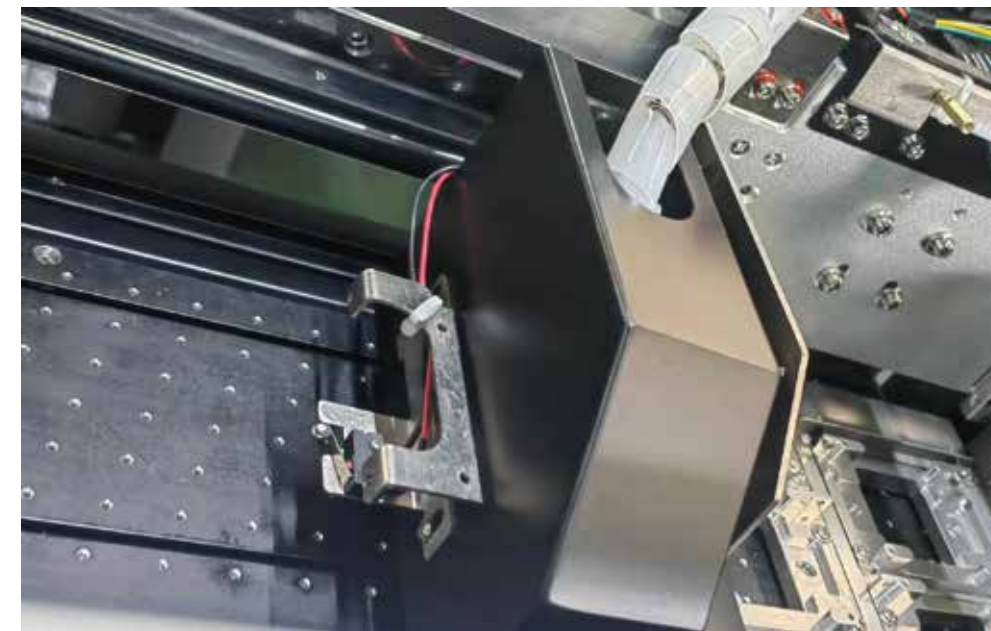
Head carriage anti-collision function
