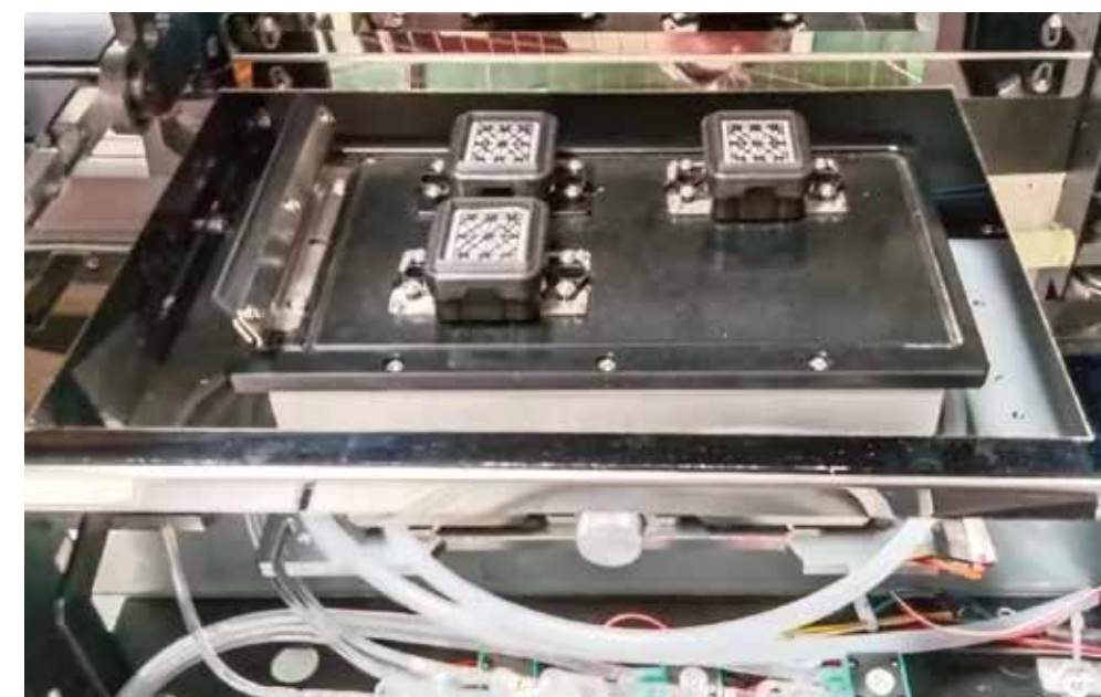
3-head ink stack configuration, flexible solution
