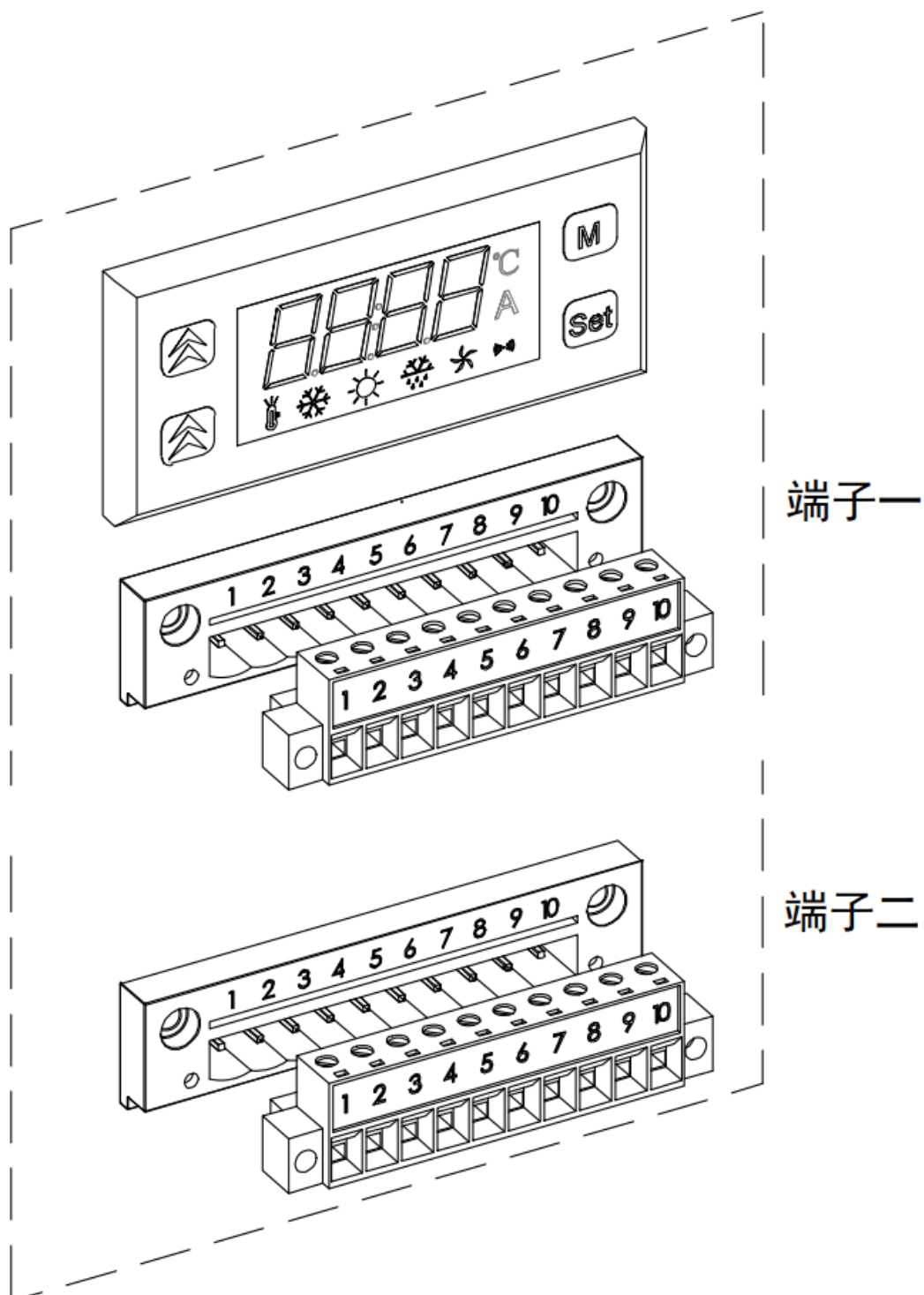
Figure6-1 Schematic of power terminal
