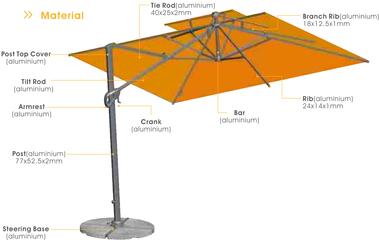
Cantilever Umbrella I Square
