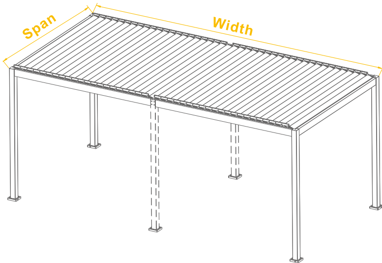
Schematic diagram of single module with 6 posts:
