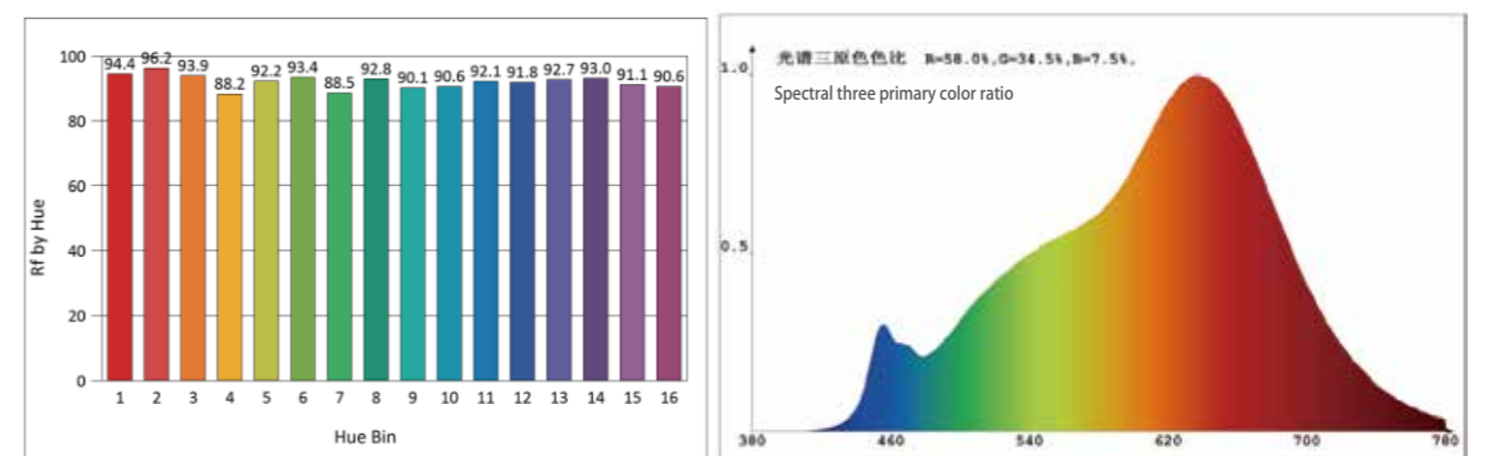
CRI>95, Color temperature: 2700K
