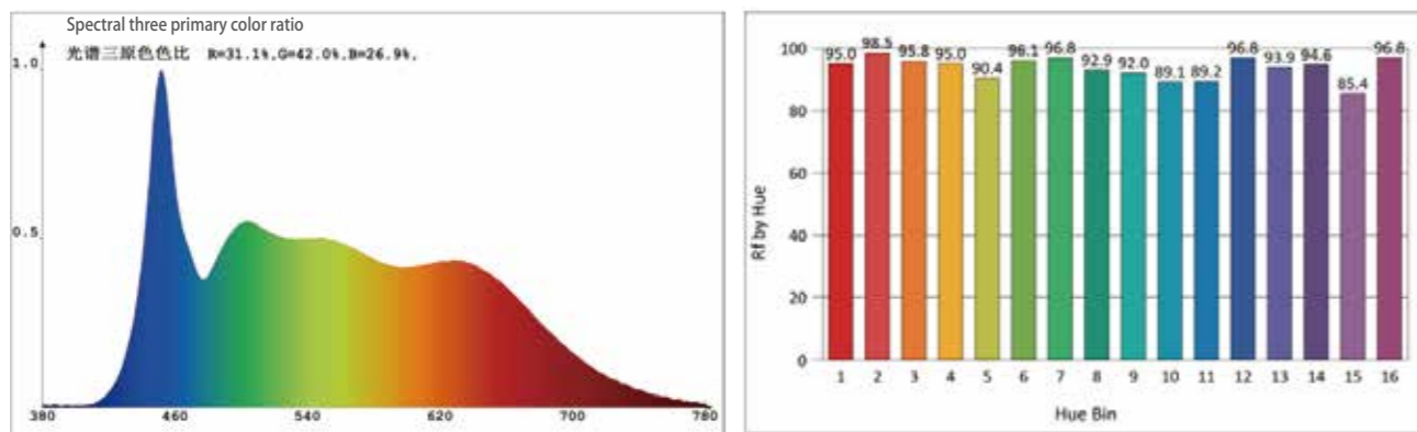
CRI>95, Color temperature: 6000K
