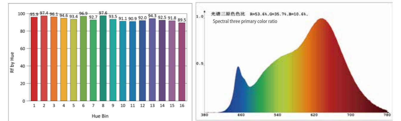
CRI>95, Color temperature: 3000K
