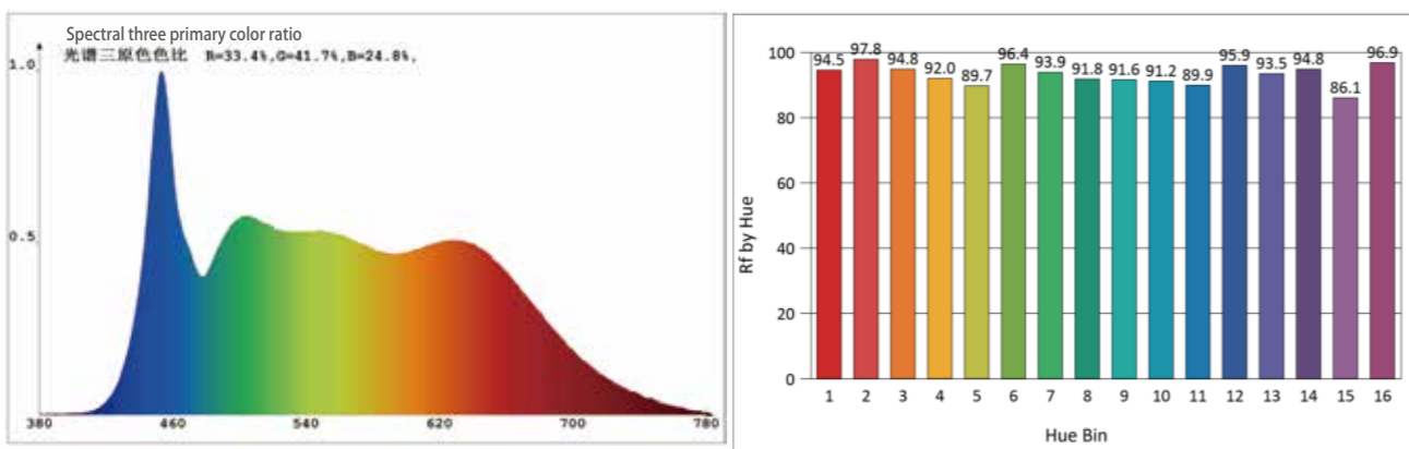
CRI>95, Color temperature: 5000K
