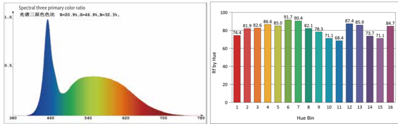
CRI>95, Color temperature: 6500K
