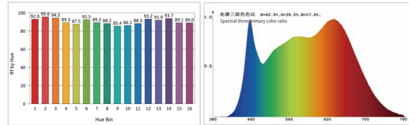
CRI>95, Color temperature: 4000K
