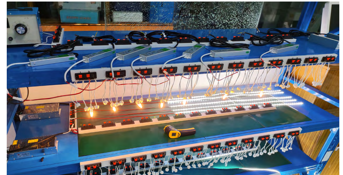
LED driver, touch switch, LED belt test machine
