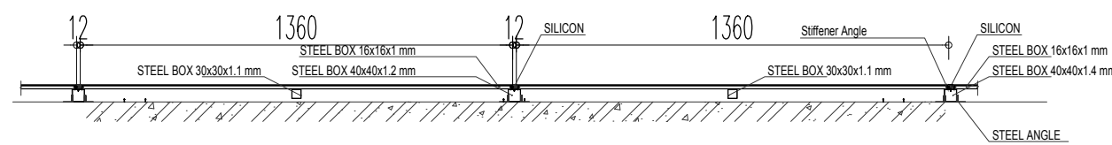
FACADE INSTALLATION (SCALE 1-20/A2)
