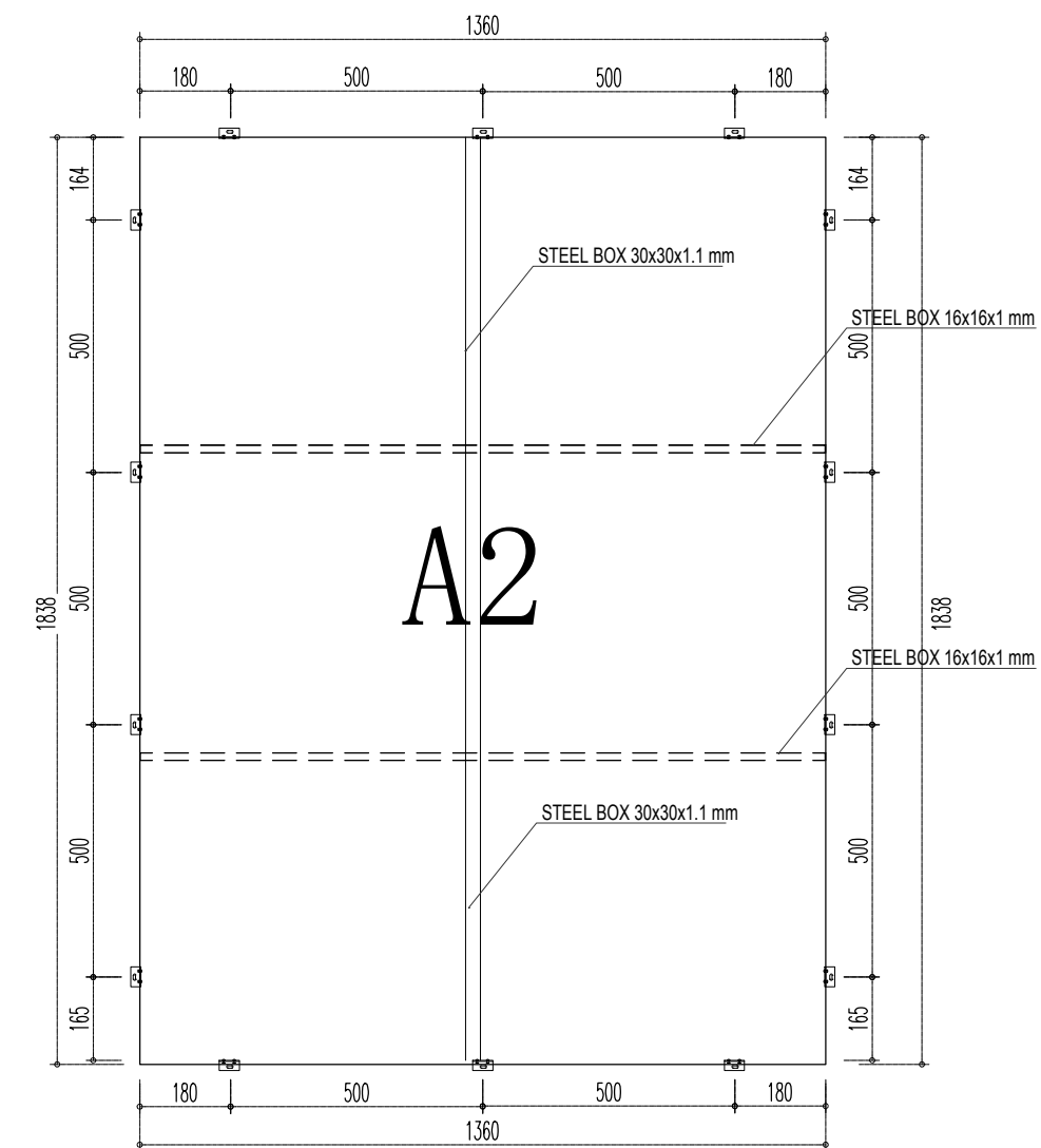
ALUMINIUM TABLE (SCALE 1-10/A2)
