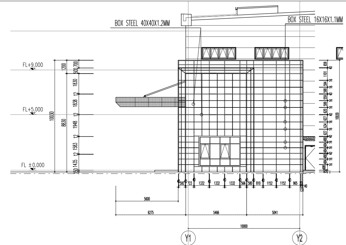
ELEVATION STEEL SUPORT FRAME AXIS X31 (Y1-Y11) (SCALE 1-200/A2)
