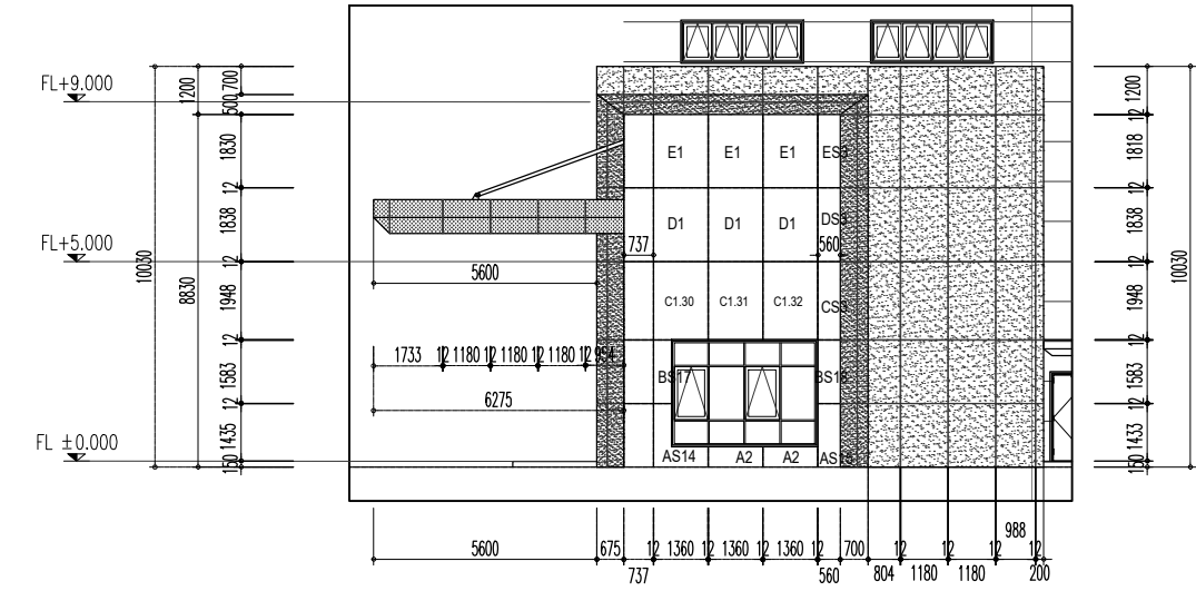
ELEVATION ALUMINUM FACADE LAYOUT DRAWING AXIS X31 (Y1-Y2) (SCALE 1-200/A2)
