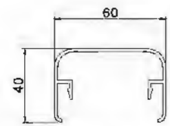
Handrail YLJ82011 T=1.7mm 0.752kg/m
