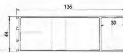
Upper Door Leaf YLJ34611 T=1.6mm 1.577kg/m
