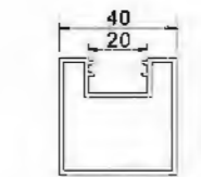
Glass Fence Crossbar YLJ82115H T=1.6mm 0.8kg/m
