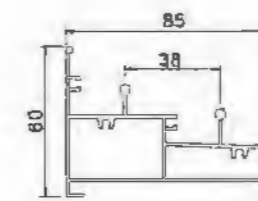
Bottom Rail YLJ188C02T T=1.45mm 1.454kg/m
