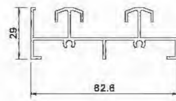
Bottom Groove L850614 T=1.4mm 0.925kg/m
