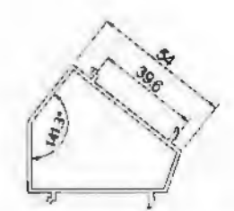
141°Corner Connecting Tube YLJ25055 T=1.4mm 0.827kg/m
