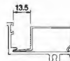
Frame Glass Bead YLJ25015K T=1.0mm 0.253kg/m
