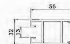
Lighting Frame L85A1920 T=2.0mm 1.015kg/m
