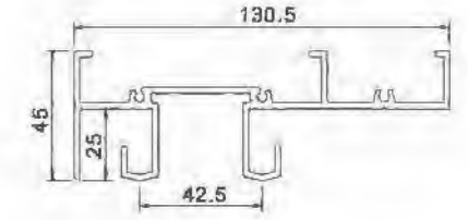
Upper Rail YLJ388A01C T=2.0mm 1.896kg/m
