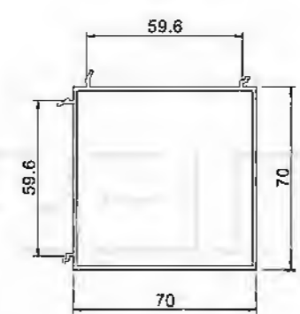
Corner Connecting Tube YLJ27007T T=1.45mm 1.17kg/m
