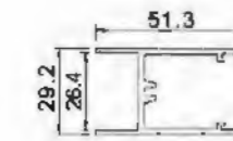
Above YLJ388A04KZK T=2.0mm 0.708kg/m
