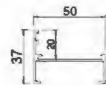
Frame YLJ25001 T=1.4mm 0.478kg/m
