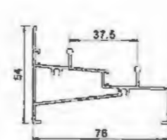
Bottom Rail YLJ180B02 T=1.2mm 0.89kg/m
