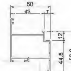
Reverse Mullion P50C2314 T=1.4mm 0.884kg/m
