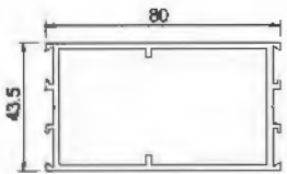
Middle Door Leaf YLJ34609B T=2.0mm 1.404kg/m
