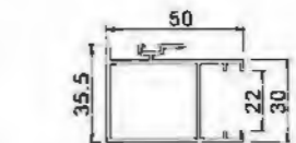
Hook Frame YLJ188C07TZK T=1.45mm 0.755kg/m
