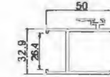
Hook Frame YLJ388A07KZK T=2.0mm 0.995kg/m
