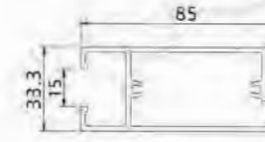
Door Leaf YLJ37015 T : 2.0mm 1.457kg/m YLJ37015C T=1.6mm 1.202kg/m
