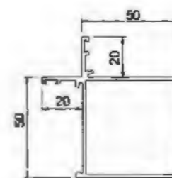
Inner Corner Frame YLJ25024P T=1.5mm 1.076kg/m
