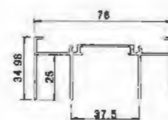
Upper Rail YLJ180B01 T=1.2mm 0.746kg/m
