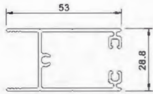
Above L850314 T=1.4mm 0.653kg/m
