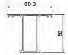
Mullion P50A0614 T=1.4mm 0.762kg/m
