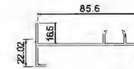
Edge Seal YLJ188C03T T=1.45mm 0.753kg/m
