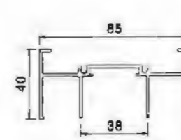
Upper Rail YLJ188C01T T=1.45mm 0.99kg/m
