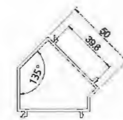
135°Corner Connecting Tube YLJ25018A T=1.7mm 0.901kg/m
