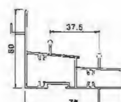
Middle Lower Rail YLJ180B02WA T=1.2mm 1.162kg/m
