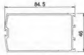
Door Leaf Vertical Frame YLJ34610 T=1.6mm 1.167kg/m
