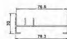
Edge YLJ180B03Z T=1.35mm 0.62kg/m
