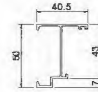
Frame P50A0314a T=1.4mm 0.498kg/m
