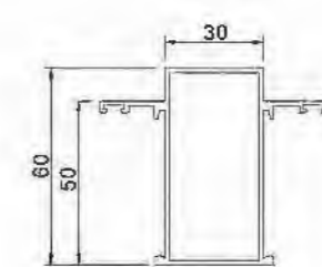
Column YLJ270D02 T=1.4mm 0.956kg/m
