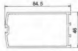
Door Leaf Vertical Frame YLJ34610A T=2.1mm 1.503kg/m
