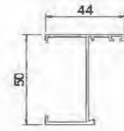
Frame P50A0314 T=1.4mm 0.507kg/m
