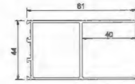
Lower Door Leaf YLJ34604 T=1.5mm 1.064kg/m
