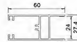
Below YLJ188C05BZK T=1.4mm 0.766kg/m
