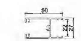
Above YLJ188C04TZK T=1.45mm 0.605kg/m
