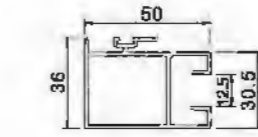
Hook Frame YLJ188C7T T=1.45mm 0.815kg/m
