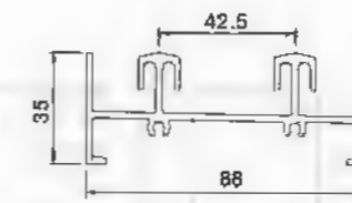
Bottom Rail YLJ388A02D T=2.0mm 1.398kg/m
