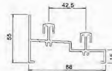
Bottom Rail YLJ388A02F T=2.0mm 1.565kg/m
