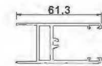
Below YLJ388A05KZK T=2.0mm 0.955kg/m
