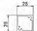
Pole YLJ82090 T=1.6mm 0.495kg/m
