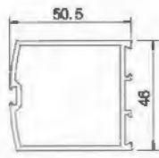
Door Leaf Vertical Frame YLJ34601H T=2.0mm 1.066kg/m
