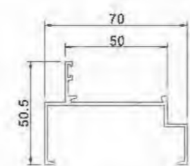
Frame YLJ270D1 T=1.4mm 0.662kg/m
