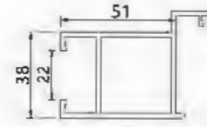
Double Sash Middle Frame YLJ37027ZK T : 2.0mm 1.223kg/m
