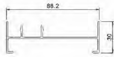
Edge L850714 T=1.4mm 0.698kg/m
