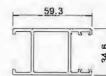
Lighting Frame L850820 T=2.0mm 1.055kg/m
