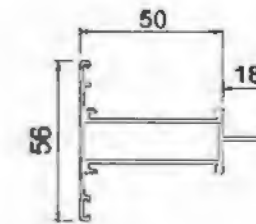
Mullion YLJ25003 T=1.4mm 0.81kg/m
