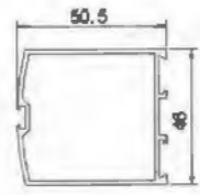
Door Leaf Vertical Frame YLJ34601 T=1.5mm 0.832kg/m
