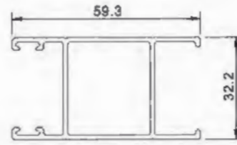
Lighting Frame L850814 T=1.4mm 0.739kg/m
