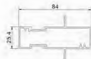
Upper Rail YLJ188A13T T=1.45mm 1.101kg/m
