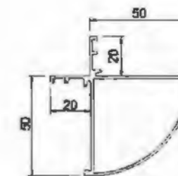
Inner Corner Frame YLJ25024D T=1.35mm 0.865kg/m
