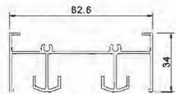
Bottom Groove L850314 T=1.4mm 1.43kg/m
