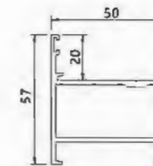
Vertical Frame YLJ35082 T : 1.9mm 1.089kg/m
