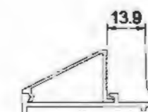
Sash Glass Bead YLJ25016 T=1.0mm 0.185kg/m
