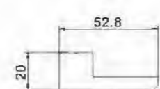
Glass Clamp YLJ01900 T=1.7mm 1.619kg/m
