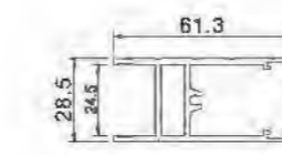
Below YLJ388A05HZK T=2.0mm 1.004kg/m
