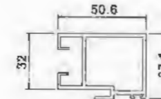
Hook Frame L85A2020 T=2.0mm 1.056kg/m
