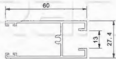
Single Tempered Glass Below L850514 T=1.4mm 0.704kg/m
