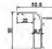
Frame YLJ25002B T=1.4mm 0.69kg/m
