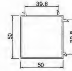
Corner Connecting Tube YLJ25011 T=1.4mm 0.85kg/m
