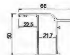
Frame YLJ25002CD T=1.4mm 0.801kg/m
