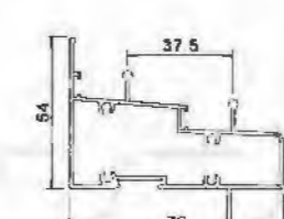
Middle Lower Rail(hollow) YLJ180B02AZK T=1.2mm 1.193kg/m
