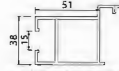
Double Sash Middle Frame YLJ37027 T : 2.0mm 1.261kg/m YLJ37027C T=1.6mm 1.031kg/m
