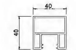
Glass Fence Crossbar YLJ82115 T=1.8mm 1.003kg/m
