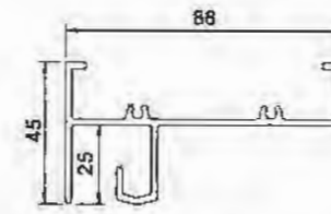
Upper Rail YLJ388A01 T=2.0mm 1.2kg/m
