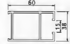
Vertical Frame YLJ37026 T : 2.0mm 1.147kg/m YLJ37026C T=1.6mm 0.939kg/m
