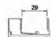
Sash Glass Bead YLJ25016B T=1.0mm 0.204kg/m
