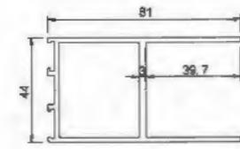
Lower Door Leaf YLJ34604A T=2.0mm 1.448kg/m
