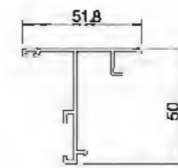
Frame Boarder Transfer Material P50C13A10 T=1.4mm 0.531kg/m
