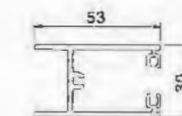
Above L850320 T=2.0mm 0.883kg/m
