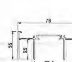
Upper Rail YLJ180B01T T=1.4mm 0.831kg/m
