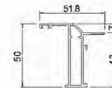
Frame P50A2714 T=1.4mm 0.669kg/m
