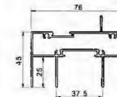
Middle Upper Rail(hollow) YLJ180B01AZK T=1.2mm 1.165kg/m
