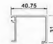
YLJ81558 T=1.4mm 0.442kg/m
