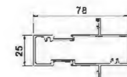
Middle Fixed Material YLJ188C13T T=1.45mm 1.037kg/m
