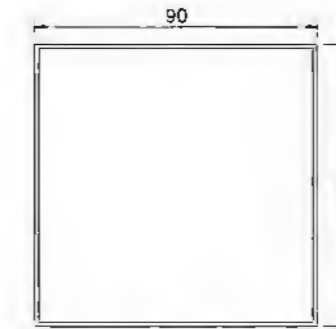
Corner Square Tube 90X90 T=1.25mm 1.211kg/m
