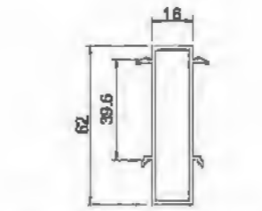
Connecting Tube YLJ25010T T=1.4mm 0.67kg/m
