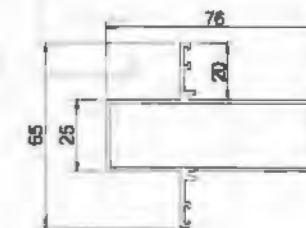
Column YLJ25023BA T=1.4mm 1.037kg/m
