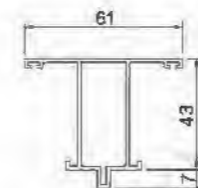
Double Open Mullion P50C0514 T=1.4mm 0.771kg/m
