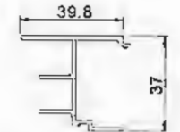
Edge Seal Close-up YLJ388A12 T=1.4mm 0.51kg/m
