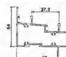
Middle Lower Rail YLJ180B02ATZK T=1.4mm 1.190kg/m
