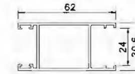
Lighting Frame YLJ188C06BZK T=1.4mm 0.768kg/m
