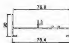
Edge YLJ180B03T T=1.4mm 0.634kg/m
