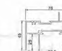
Middle Upper Rail YLJ180B01AT T=1.4mm 1.329kg/m
