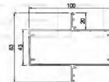
Strengthen Column YLJ25023A T=1.4mm 1.423kg/m
