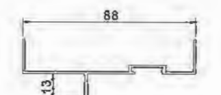
Edge Seal Cover YLJ388A17 T=2.0mm 0.489kg/m
