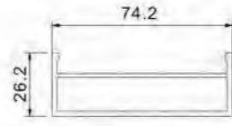
Handrail Base YLJ82093 T=2.2mm 1.028kg/m
