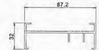
Edge Frame L85A1020 T=2.0mm 0.968kg/m
