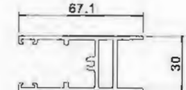
Below L850520 T=2.0mm 1.152kg/m
