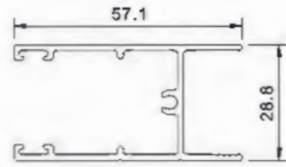
Below L850414 T=1.4mm 0.631kg/m
