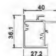
JHB7004 T=1.45mm 0.650kg/m
