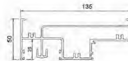
Upper Rail YLJ313501 T=2.0mm 2.558kg/m
