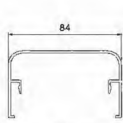
Handrail YLJ82099 T=1.7mm 0.966kg/m
