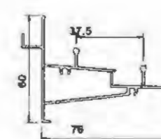
Bottom Rail YLJ180B02W T=1.2mm 0.944kg/m
