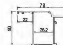
Frame YLJ25002CDA T=1.4mm 0.844kg/m
