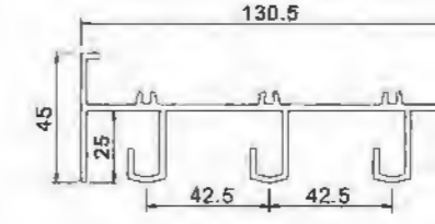
Upper Rail YLJ388A01G T=2.0mm 2.097kg/m
