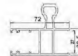
Handles Of Doors And Windows YLJ313506 T=2.0mm 1.664kg/m
