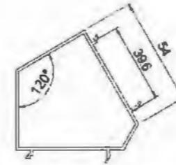
120°Corner Connecting Tube YLJ25018T T=1.4mm 0.832kg/m
