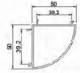
Corner Connecting Tube YLJ25011BT T=1.4mm 0.742kg/m
