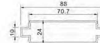
Connecting Tube YLJ188C10 T=1.4mm 0.895kg/m
