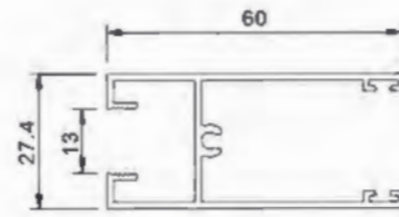
Single Tempered Glass Above L85A1714 T=1.4mm 0.704kg/m
