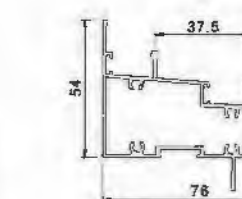
Middle Bottom Rail YLJ180B02A T=1.2mm 1.101kg/m
