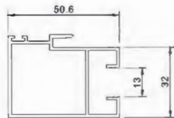
Hook Frame L85A2014 T=1.4mm 0.798kg/m
