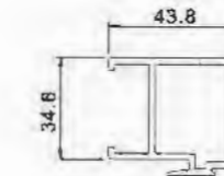
Hook Frame L850920 T=2.0mm 0.942kg/m
