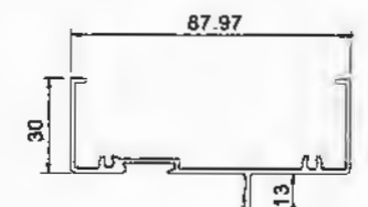
Above Fixed YLJ18810T T=1.45mm 0.767kg/m
