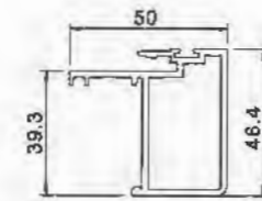
Fixed Hook Frame YLJ388A07A T=2.0mm 1.005kg/m
