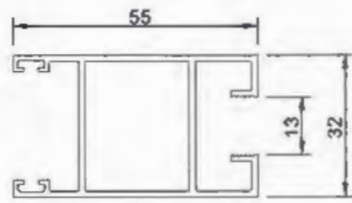
Lighting Frame L85A1914D T=1.4mm 0.771kg/m
