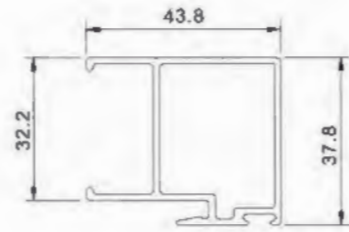
Hook Frame L850914 T=1.4mm 0.665kg/m
