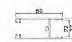
Inner Below YLJ188C05TZK T=1.45mm 0.683kg/m
