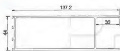
Upper Door Leaf YLJ34611H T=2.0mm 1.97kg/m
