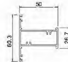
Mullion P50A3714 T=1.4mm 0.826kg/m
