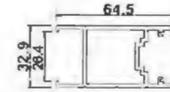
Lighting Frame YLJ388A06KZK T=2.0mm 1.128kg/m
