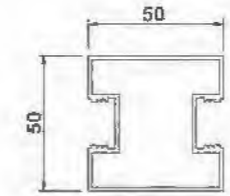
Column FS-003 T=1.4mm 0.968kg/m
