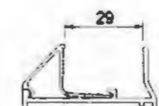
Sash Glass Bead YLJ25016R T=1.0mm 0.187kg/m
