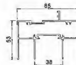
Middle Upper Rail YLJ188C01AT T=1.45mm 1.565kg/m
