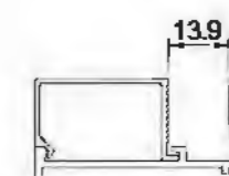
Sash Glass Bead YLJ25016M T=1.0mm 0.211kg/m
