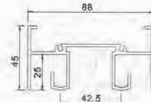
Upper Rail YLJ388A01B T=2.0mm 1.633kg/m
