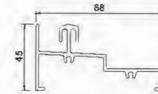
Upper Rail YLJ388A02 T=2.0mm 1.248kg/m
