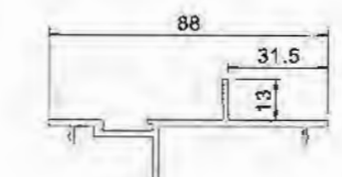
Upper Rail Cover YLJ388A13 T=2.0mm 10.708kg/m
