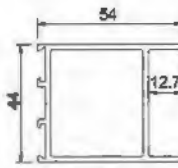
Upper Door Leaf YLJ34603H T=2.0mm 1.061kg/m
