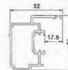
Sash Close-up YLJ35108 T : 1.6mm 0.998kg/m
