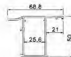
Sash YLJ313516 T=1.6mm 0.927kg/m
