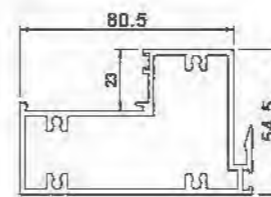
Fixed Column YLJ313504 T=2.0mm 1.948kg/m
