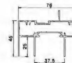
Middle Upper Rail YLJ180B01A T=1.2mm 1.163kg/m
