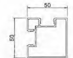
Corner Column FS-004 T=1.4mm 0.995kg/m
