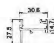
JHB7007 T=1.45mm 0.363kg/m
