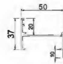
Frame YLJ25006 T=1.4mm 0.51kg/m
