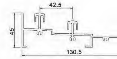
Bottom Rail YLJ388A02C T=2.0mm 1.918kg/m
