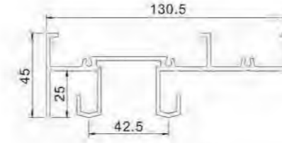
Upper Rail YLJ388A01C T=2.0mm 1.896kg/m
