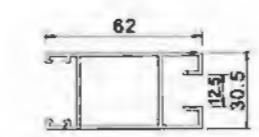
Lighting Frame YLJ188C06T T=1.45mm 0.847kg/m
