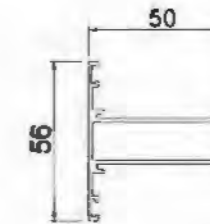
Mullion YLJ25004 T=1.4mm 0.766kg/m
