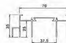
Upper Rail YLJ180B01W T=1.2mm 0.828kg/m
