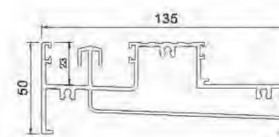
Bottom Rail YLJ313502 T=2.0mm 2.519kg/m
