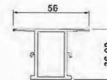
Fixed Middle Mullion L85A1120 T=2.0mm 0.816kg/m
