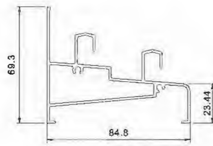
Bottom Groove L850614 T=1.4mm 1.323kg/m
