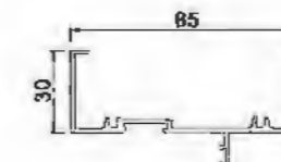
Upper Fixed Material YLJ188C14T T=1.45mm 0.774kg/m
