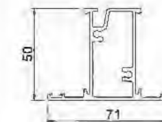
Fixed Middle YLJ313515 T=1.6mm 1.116kg/m
