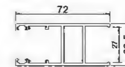
Doors And Windows YLJ313505 T=2.0mm 1.188kg/m
