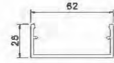
Fence Crossbar YLJ82094 T=2.2mm 0.685kg/m
