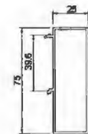
Connecting Tube YLJ25010C T=1.4mm 0.839kg/m
