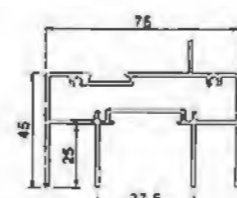
Middle Upper Rail(hollow) YLJ180B01ATZK T=1.4mm 1.1229kg/m
