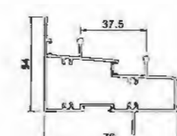
Middle Lower Rail YLJ180B02AT T=1.4mm 1.198kg/m
