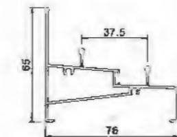
Bottom Rail YLJ180B02C T=1.2mm 0.91kg/m
