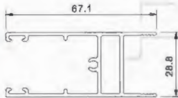
Below L850514 T=1.4mm 0.807kg/m
