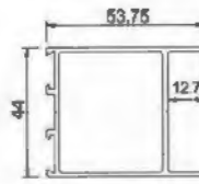
Upper Door Leaf YLJ34603 T=1.5mm 0.844kg/m
