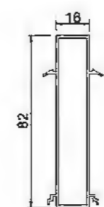
Connecting Tube YLJ27008 T=1.26mm 0.748kg/m
