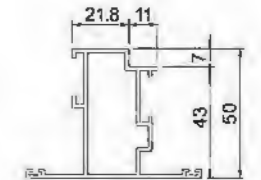
Frame P50C2814 T=1.4mm 0.877kg/m
