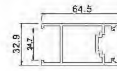
Lighting Frame YLJ388A06HZK T=2.0mm 1.164kg/m
