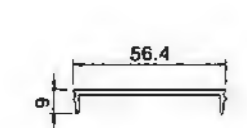
Fence Crossbar Seal Cover YLJ82095 T=2.0mm 0.358kg/m
