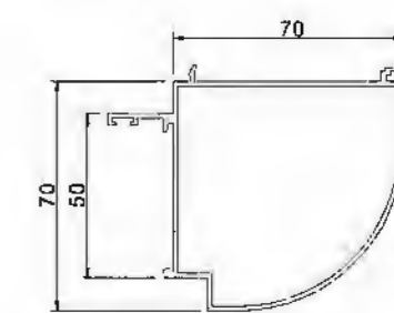
Corner Material YLJ270D03 T=1.35mm 1.123kg/m
