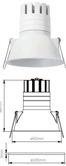
GE-05101-8W-105-H27K90WH
