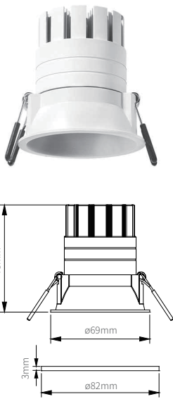
GE-05100-8W-82-H27K90WH
