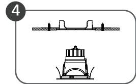
Press the spring plate and push the lamp into the hole
