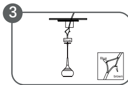
Connect the AC wires and Driver's Input wires
